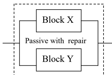
Figure 9 Passive redundancy - with repair
