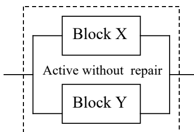
Figure 10 Active redundancy - without repair when only one block has failed
