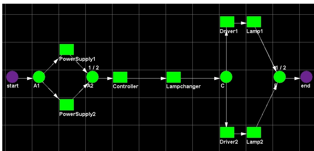
Figure 13 Reliability Block Diagram of Typical AtoN
