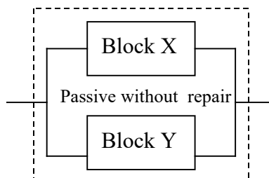
Figure 7 Passive redundancy - without repair
