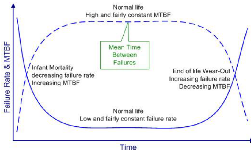
Figure 3 MTBF is only constant during the so-called normal part of the life cycle
