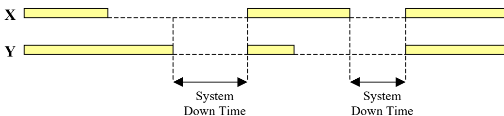
Figure 12 Presentation of active redundancy - with repair
