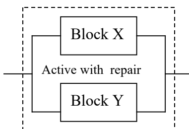
Figure 11 Active redundancy - with repair when only one block has failed
