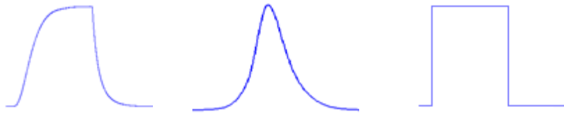
Figure 1 Typical flash shapes (pulse profiles) produced by flashing incandescent light sources (left), any light sources in rotating optics (middle), and rectangular LED pulse (right)
