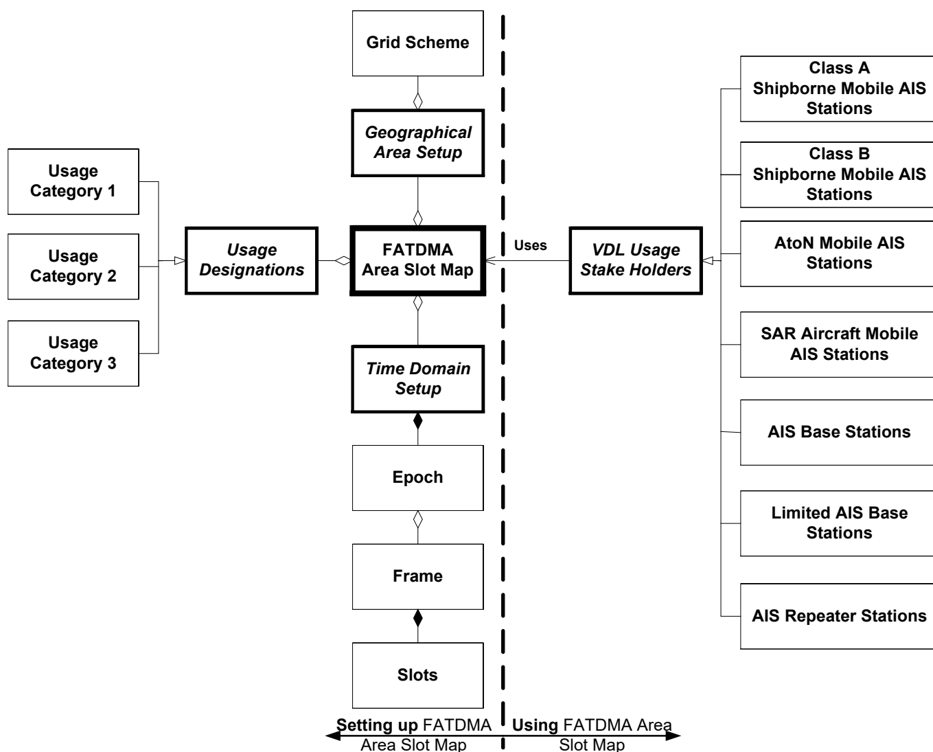
Figure 1 FATDMA Area slot map
