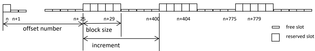
Figure 4 Example for one FATDMA reservation within a Data Link Management message transmitted in Message-20-slot n
