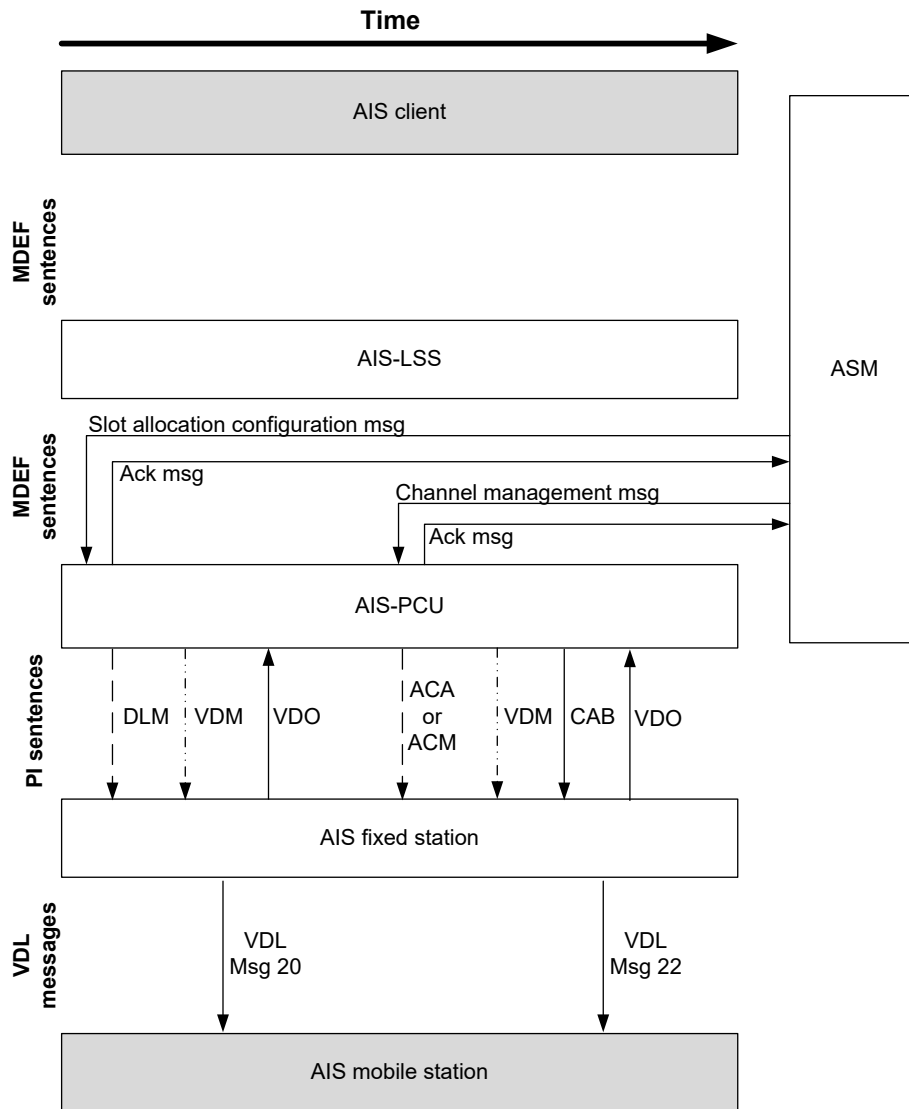
Figure 24 Interaction & data flow model for internal BAS FATDMA and CH_MGMT
