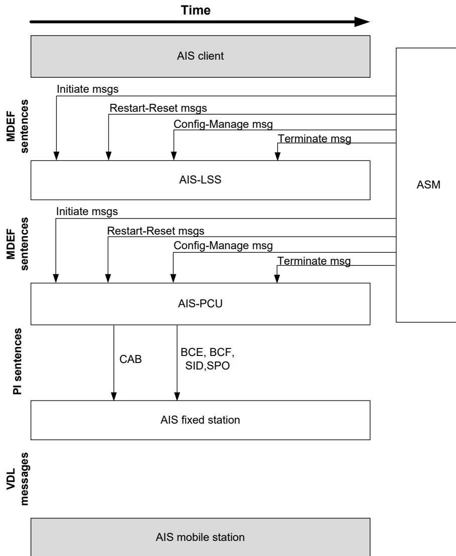
Figure 22 Interaction & data flow model for internal BAS INIT_AIS, TERM_AIS, LSS_MGMT, PCU_MGMT and STA_MGMT.
