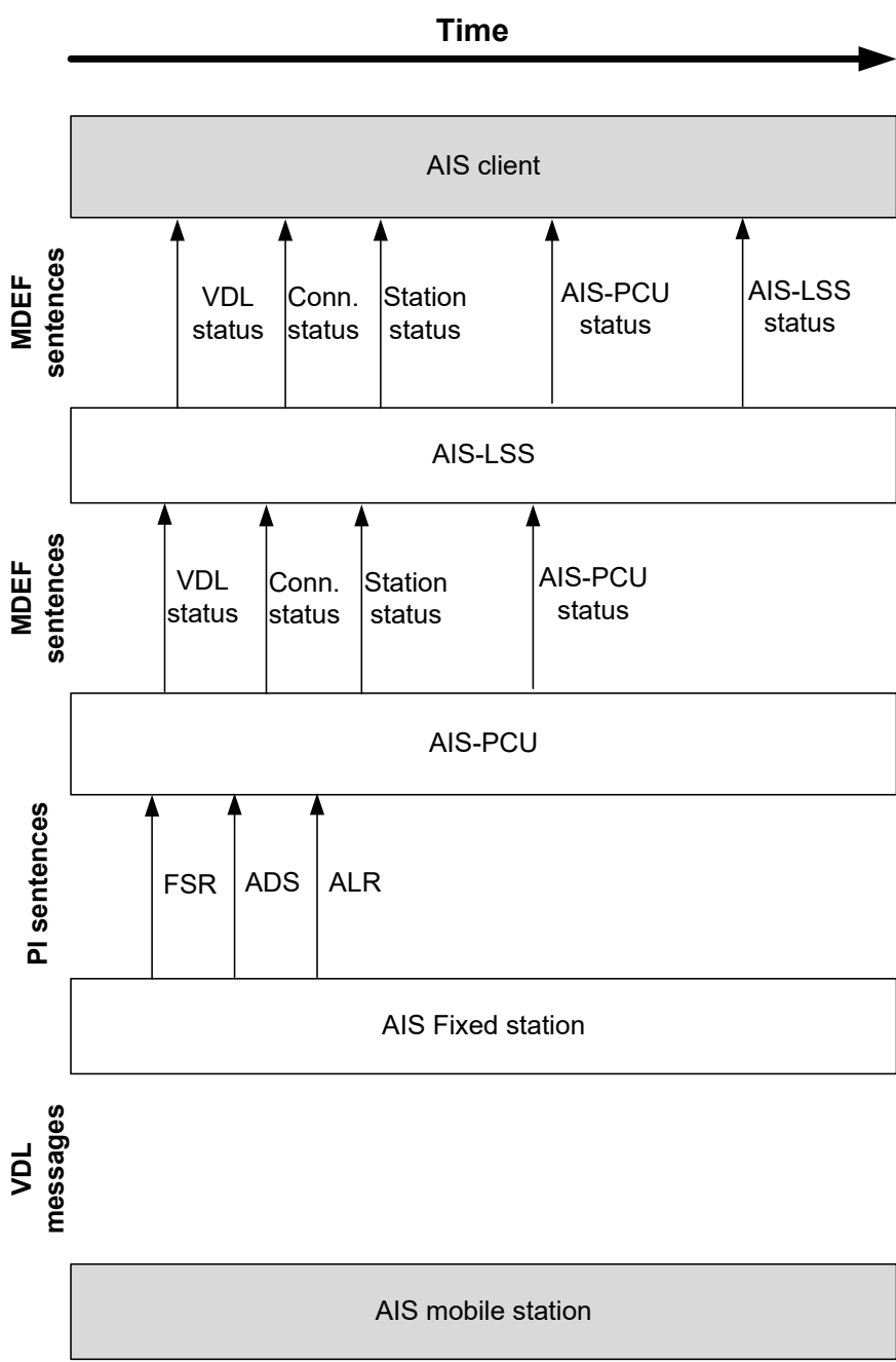
Figure 20 Interaction & data flow model for external BAS AIS_MON
