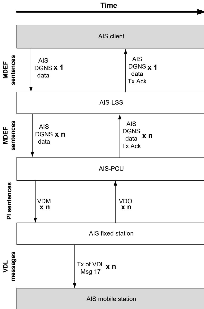
Figure 16 Interaction & data flow model for external BAS DGNS_COR
