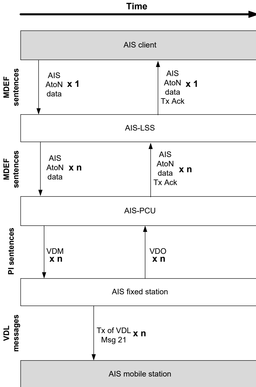
Figure 10 Interaction & data flow model for external BAS ATON_DAT in Tx mode
