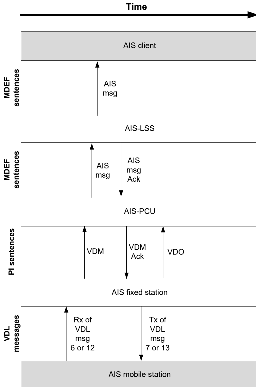
Figure 12 Interaction & data flow model for external BAS ASC_AD, SAFE_AD in Rx mode when addressed to MMSI of AIS client
