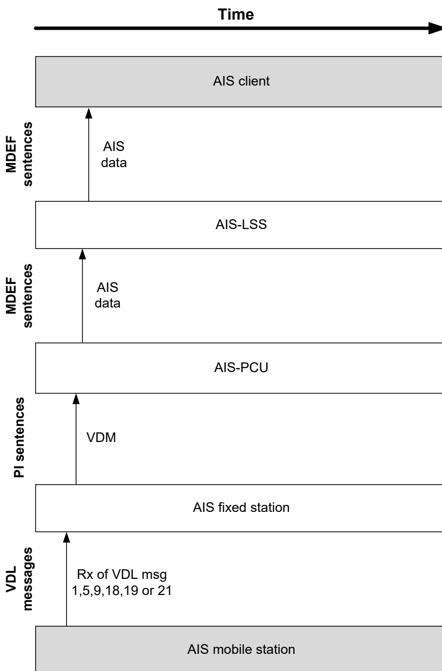
Figure 8 Interaction & data flow model for external BAS A_DYN, A_STAT, A_VOY, B_DAT, SAR_DAT, SART_DAT, STA_PROFILE
