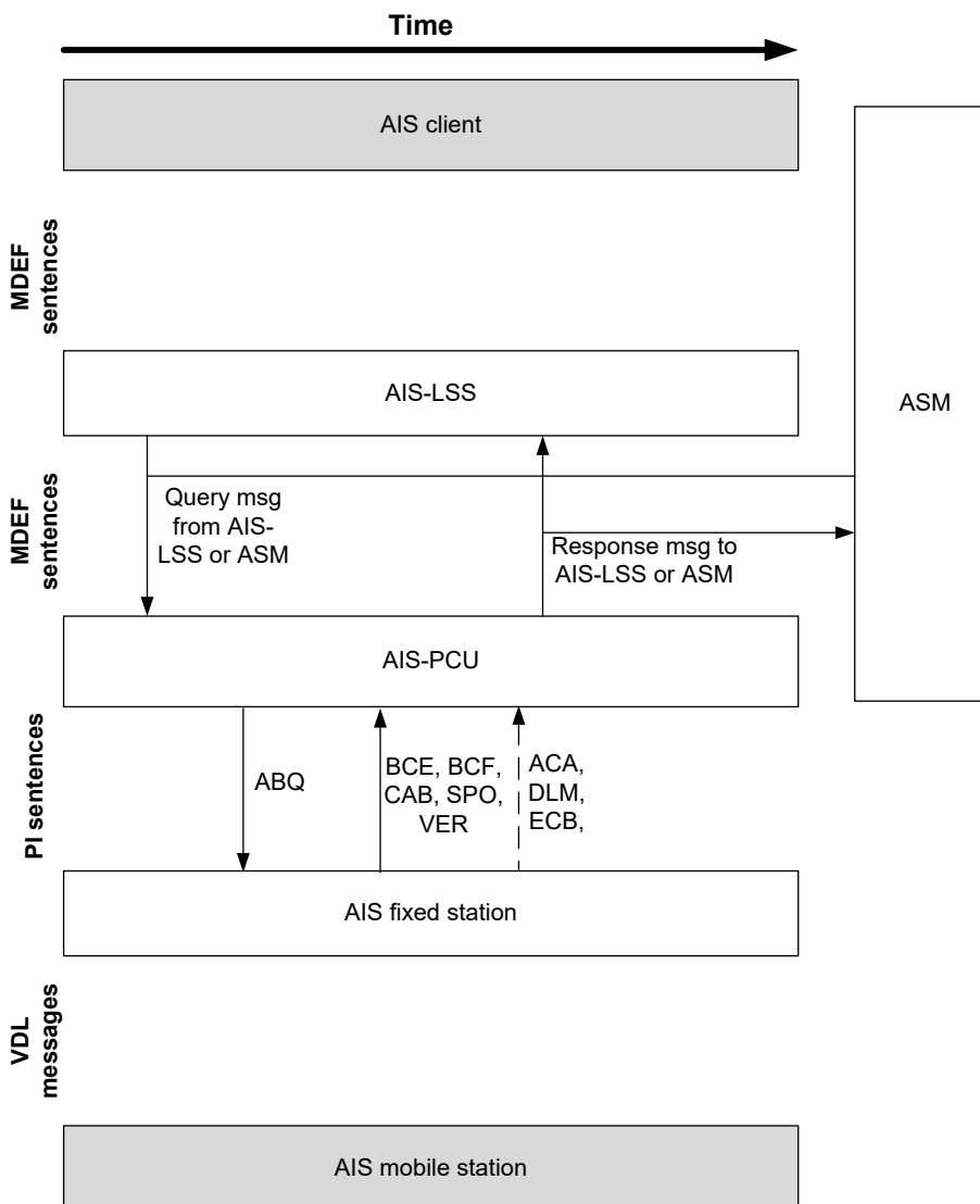
Figure 23 Interaction & data flow model for internal BAS BASE_DAT
