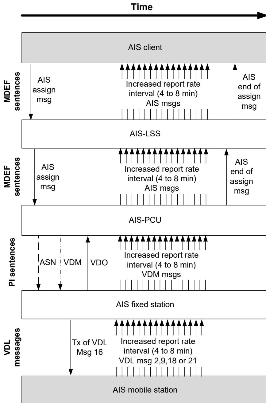
Figure 18 Interaction & data flow model for external BAS ASGN_RATE
