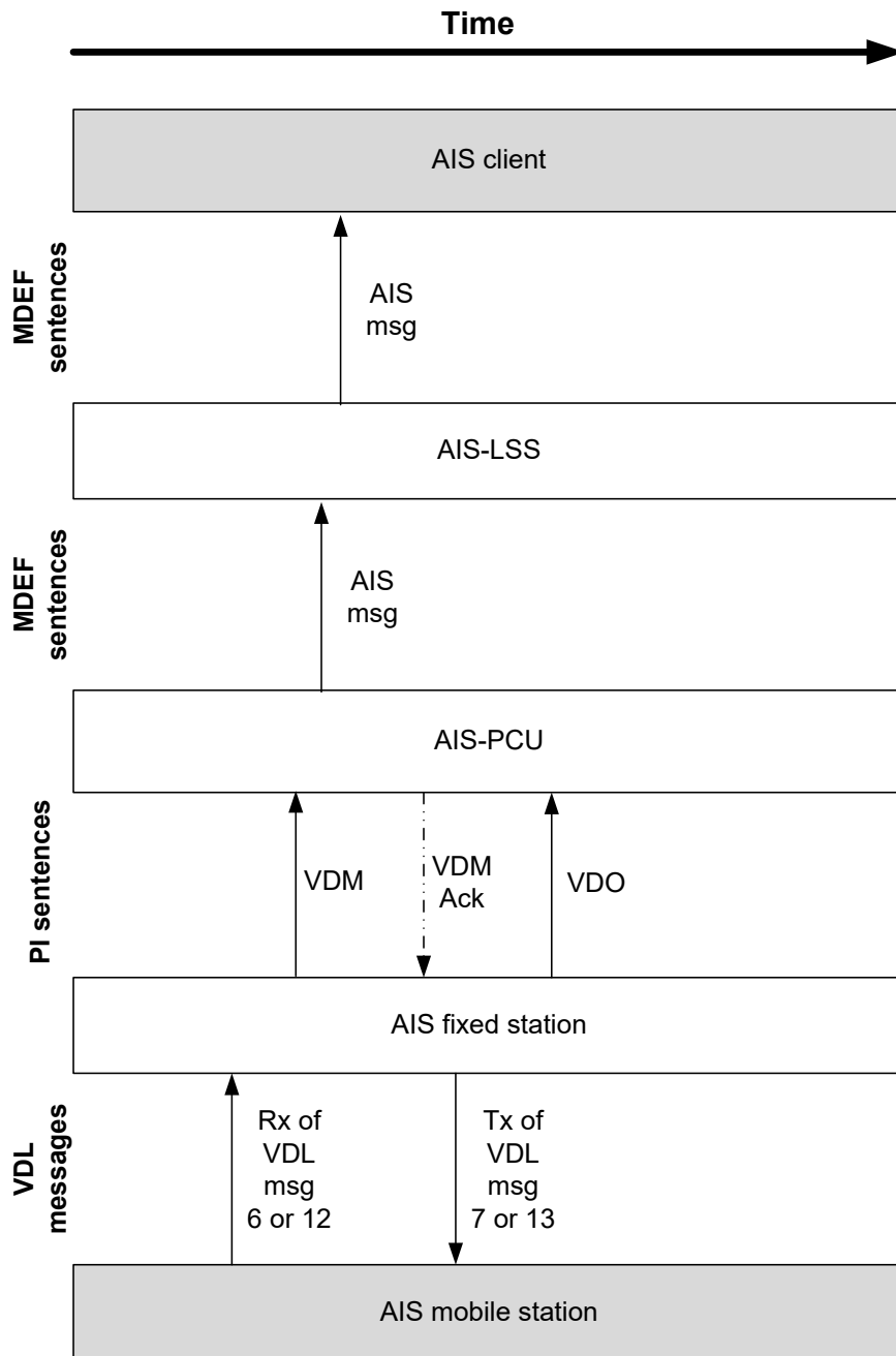
Figure 11 Interaction & data flow model for external BAS ASC_AD, SAFE_AD in Rx mode when addressed to MMSI of fixed station
