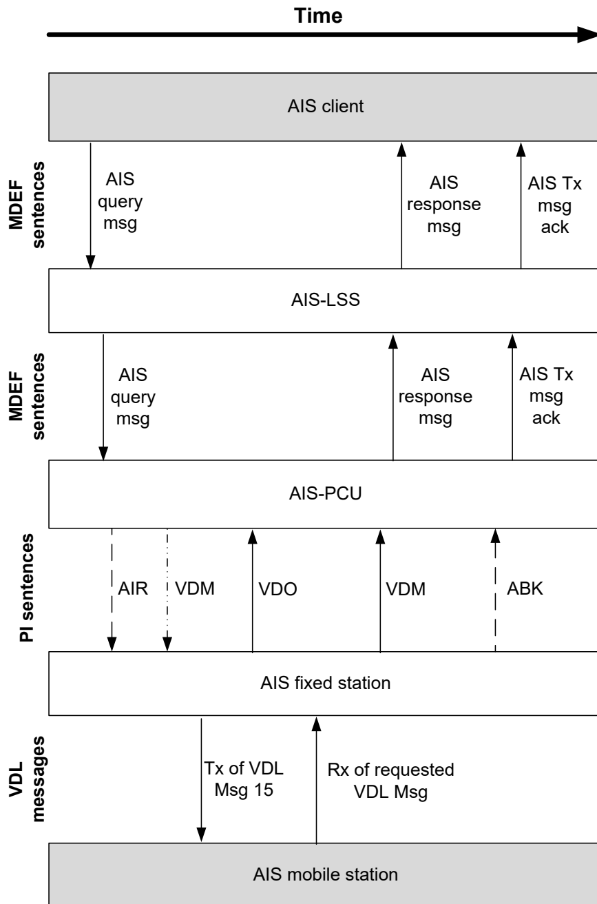
Figure 17 Interaction & data flow model for external BAS INT_TDMA
