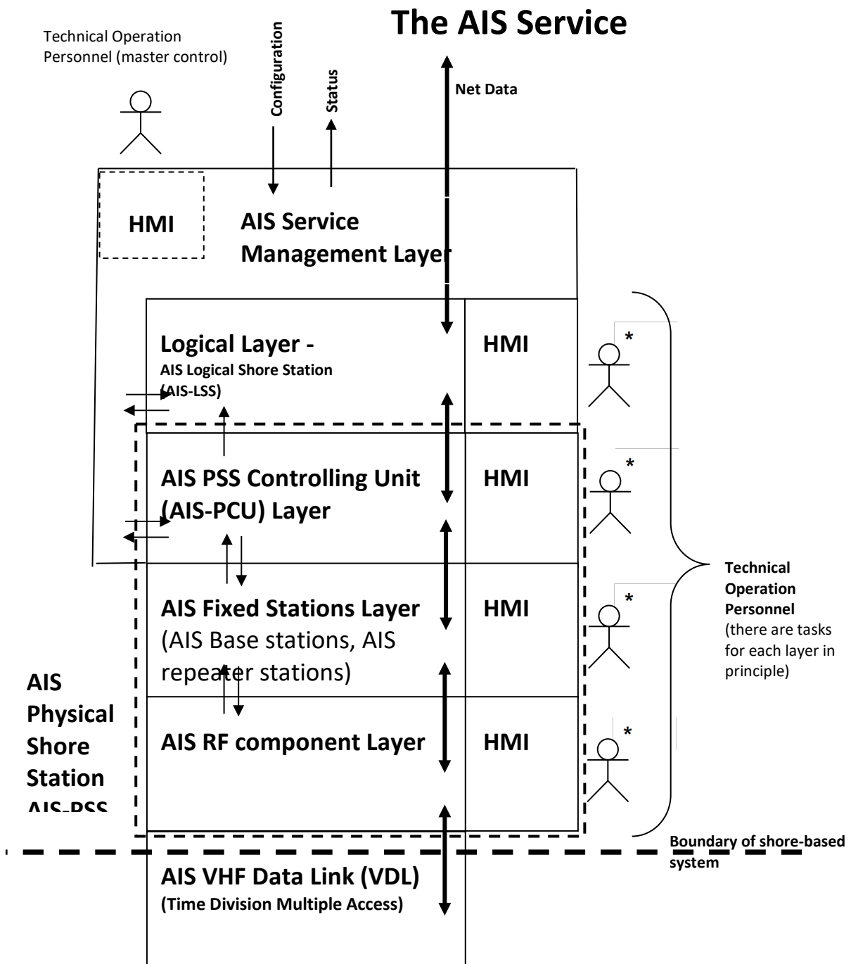
Figure 1 Layered structure of AIS Service – Structure model of the AIS Service
