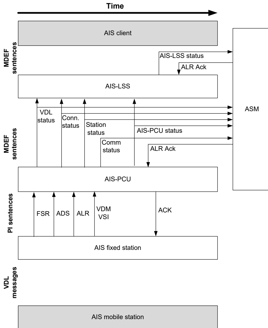
Figure 25 Interaction & data flow model for internal BAS AIS_MON
