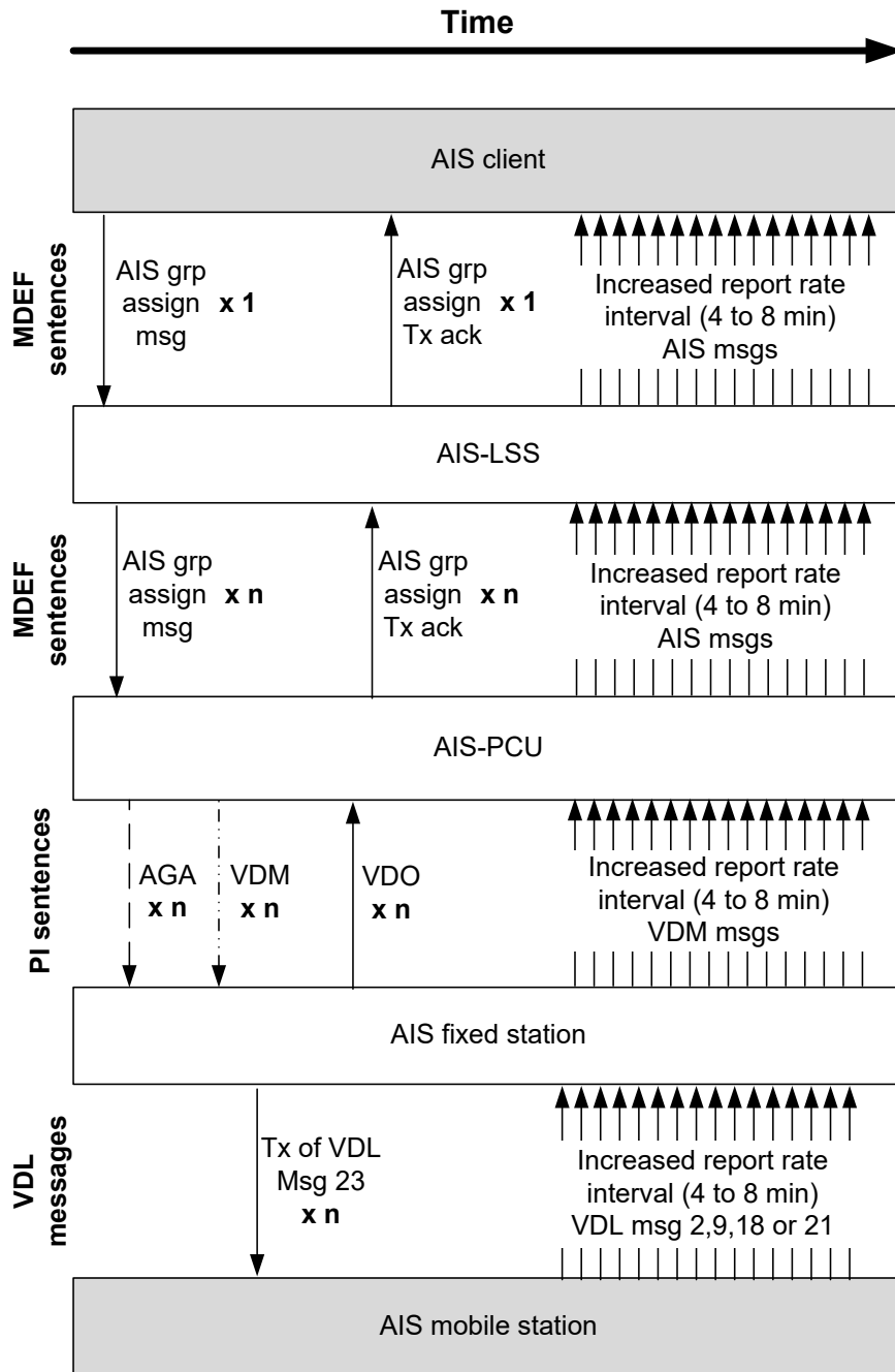
Figure 19 Interaction & data flow model for external BAS ASGN_GROUP
