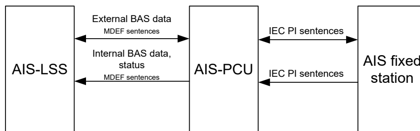
Figure 3 Interactions between AIS-PCU and AIS-LSS
