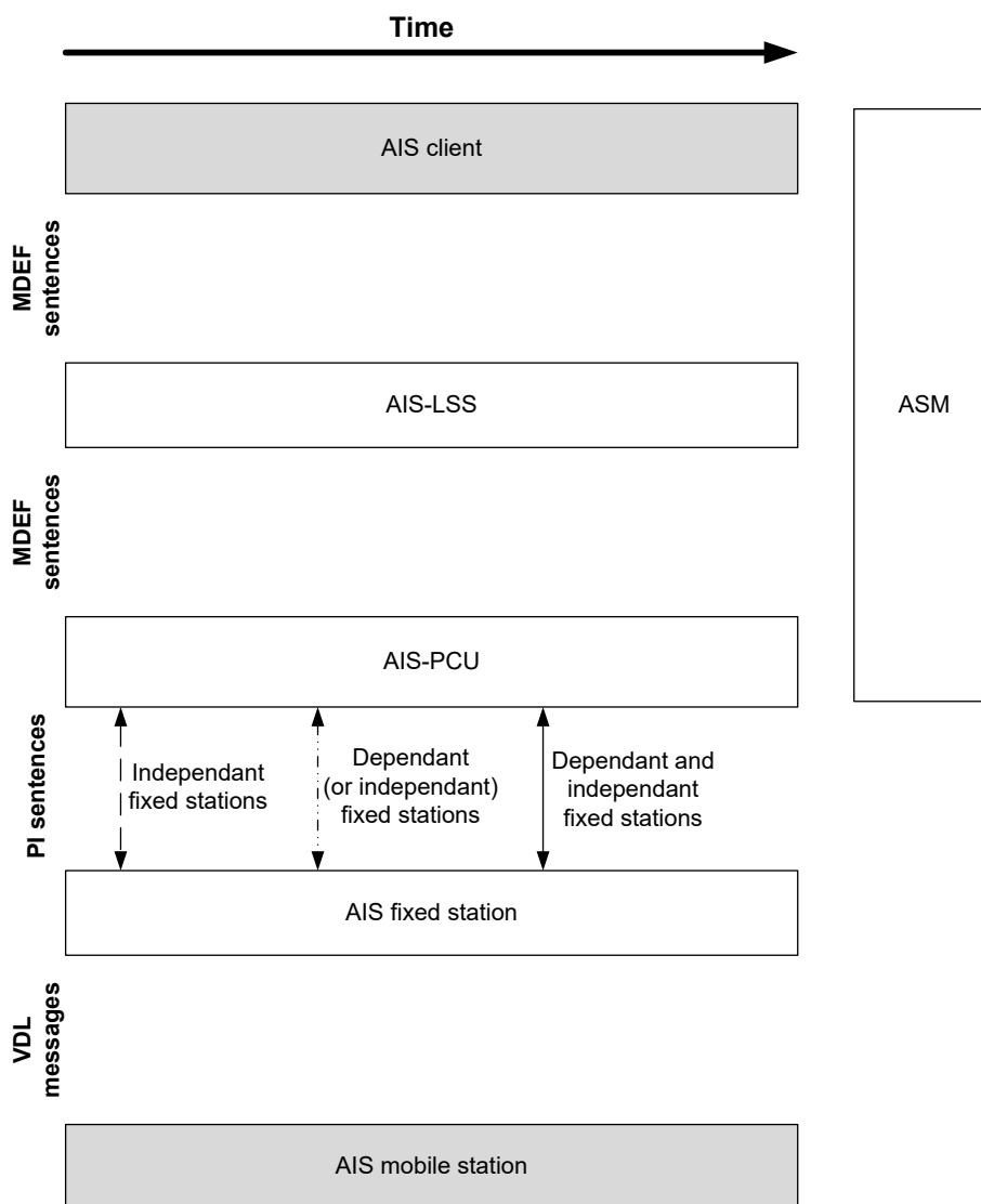
Figure 21 Template for internal BAS interaction & data flow model
