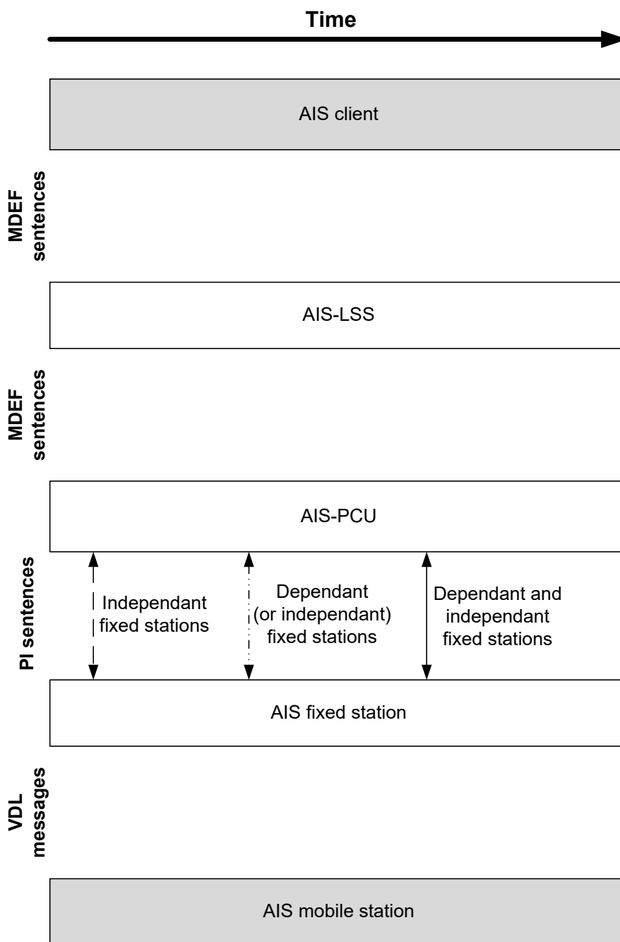
Figure 7 Template for external BAS interaction & data flow model
