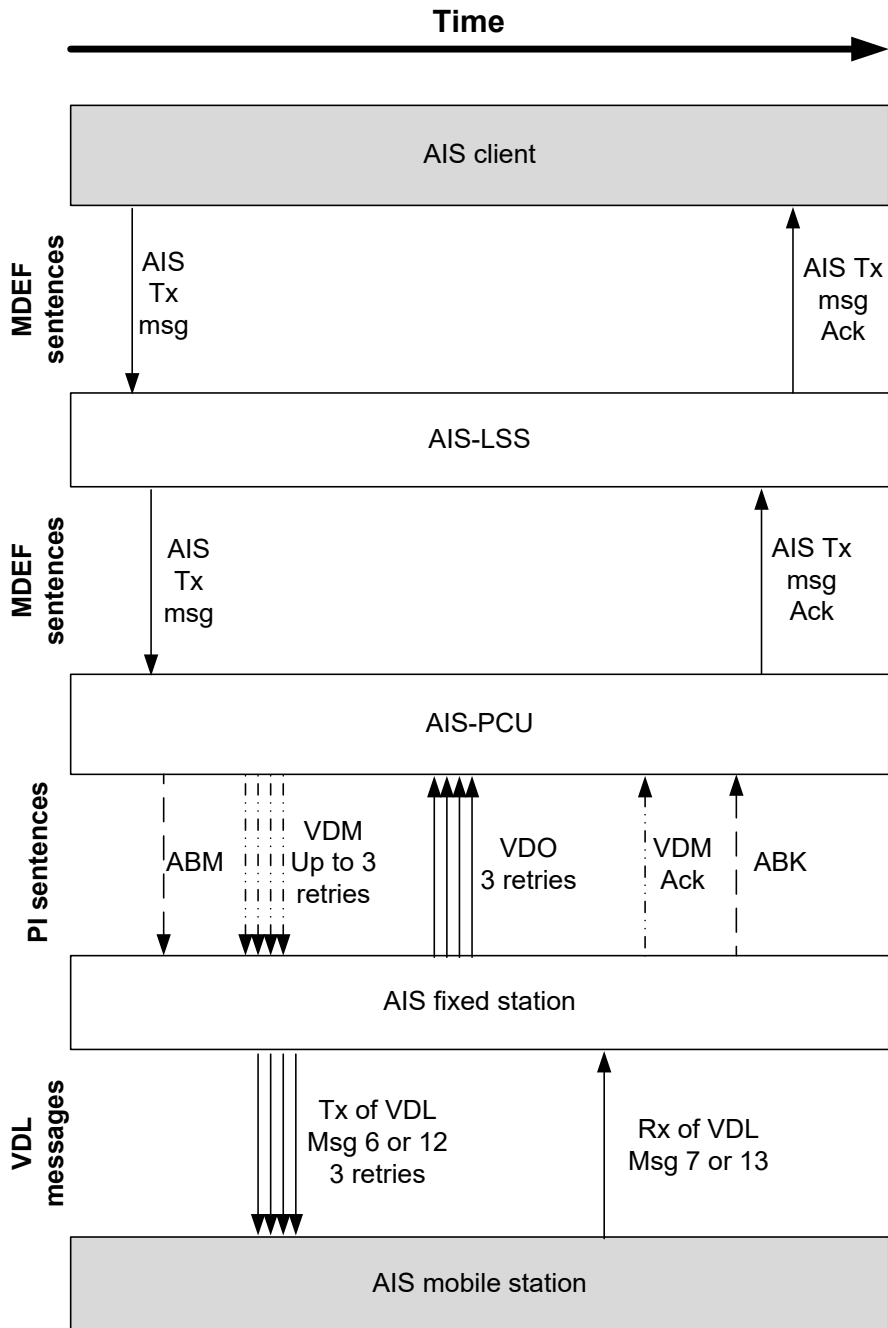
Figure 13 Interaction & data flow model for external BAS ASC_AD, SAFE_AD in Tx mode
