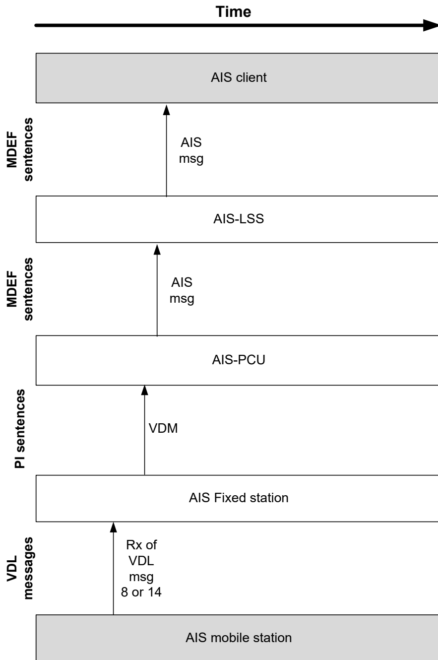
Figure 14 Interaction & data flow model for external BAS ASC_BR, SAFE_BR in Rx mode
