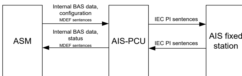
Figure 4 Interactions between AIS-PCU and ASM
