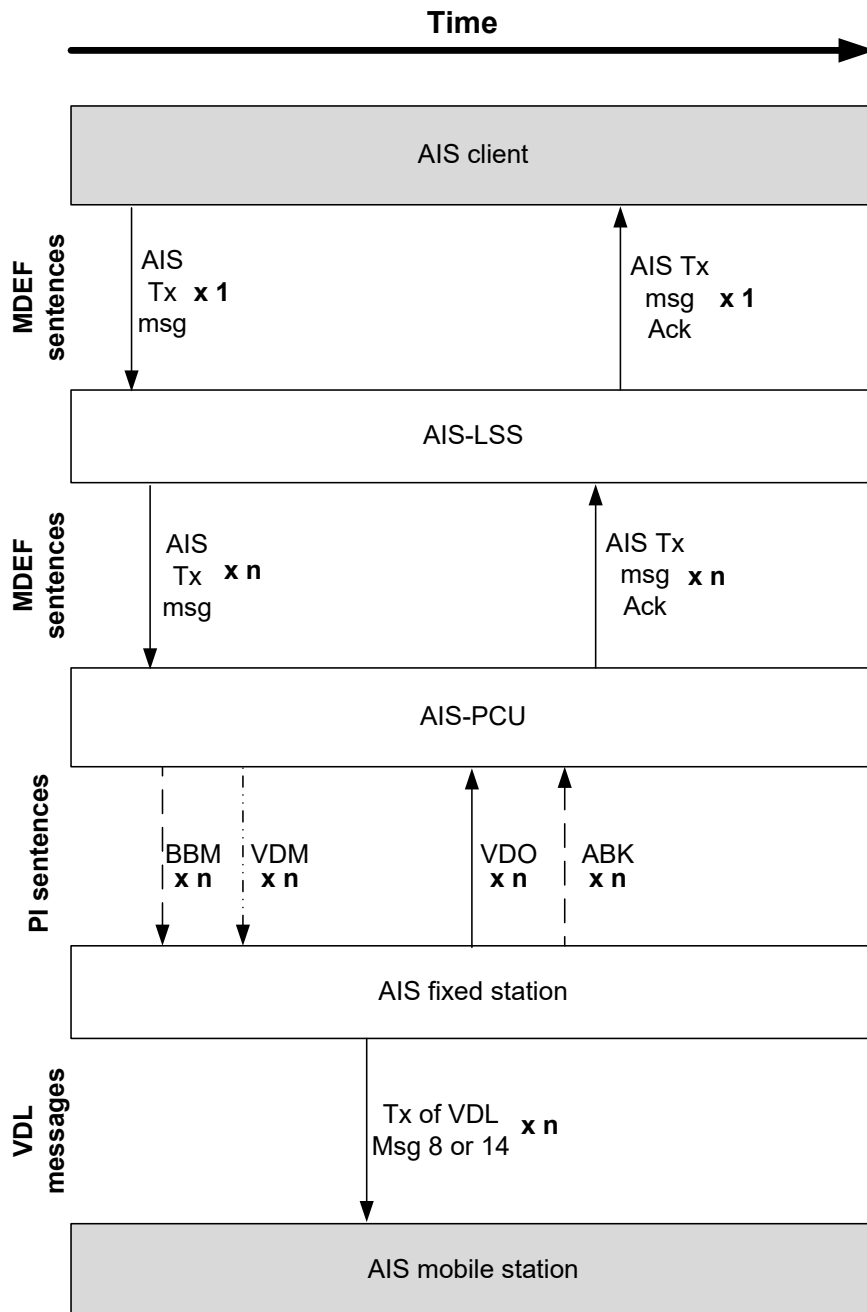
Figure 15 Interaction & data flow model for external BAS ASC_BR, SAFE_BR in Tx mode
