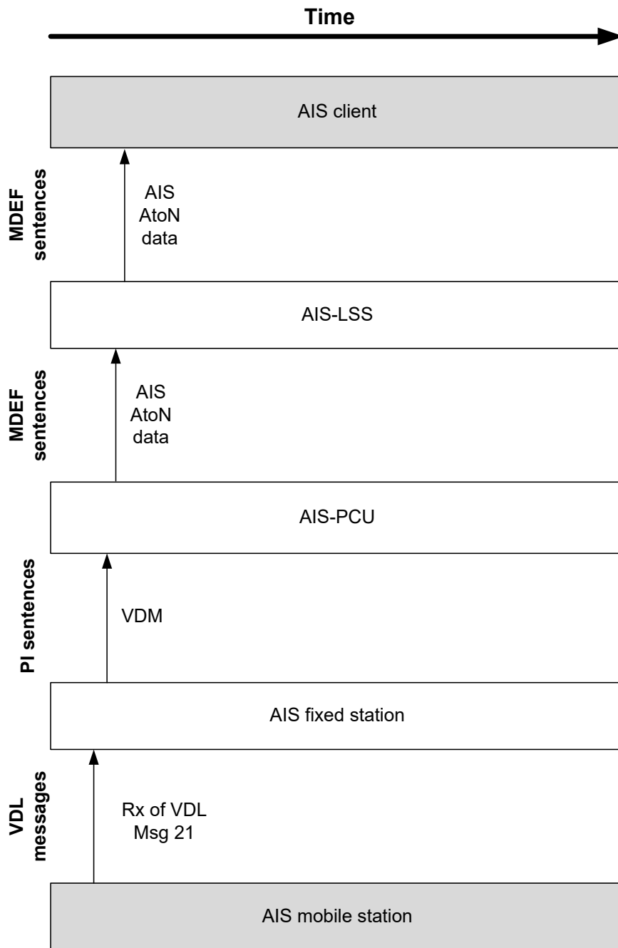
Figure 9 Interaction & data flow model for external BAS ATON_DAT in Rx mode
