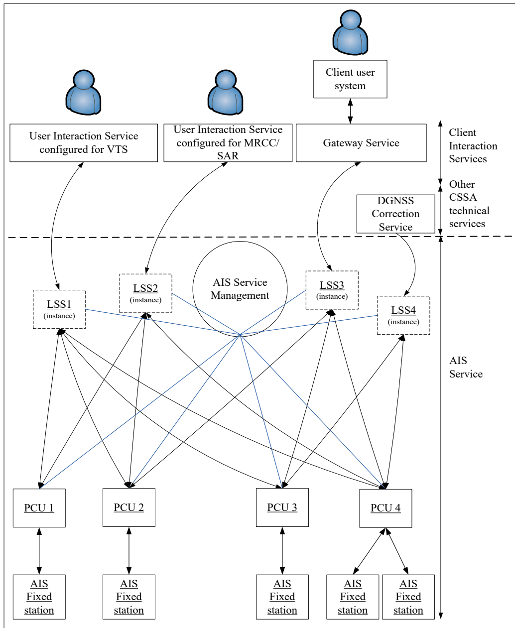
Figure 2 Example of interactions within an AIS Service and with other shore-based services
